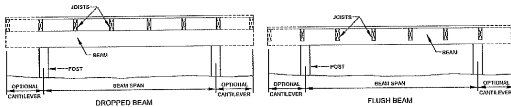
FIGURE R507.6 TYPICAL DECK BEAM SPANS
