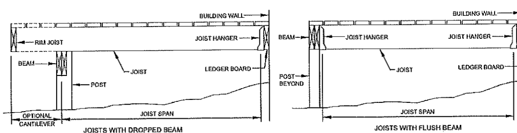
FIGURE R507.5 TYPICAL DECK JOIST SPANS
